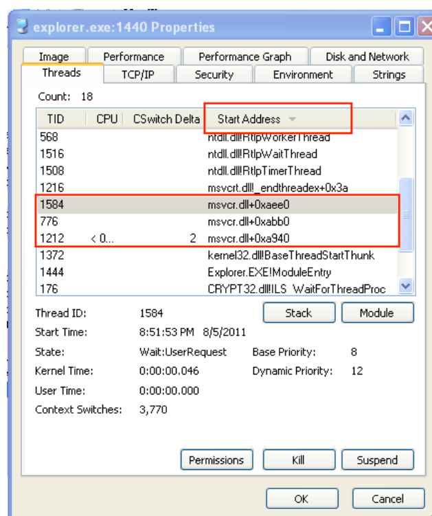
Figure 6. Three additional threads was indentied by using Process Explorer
